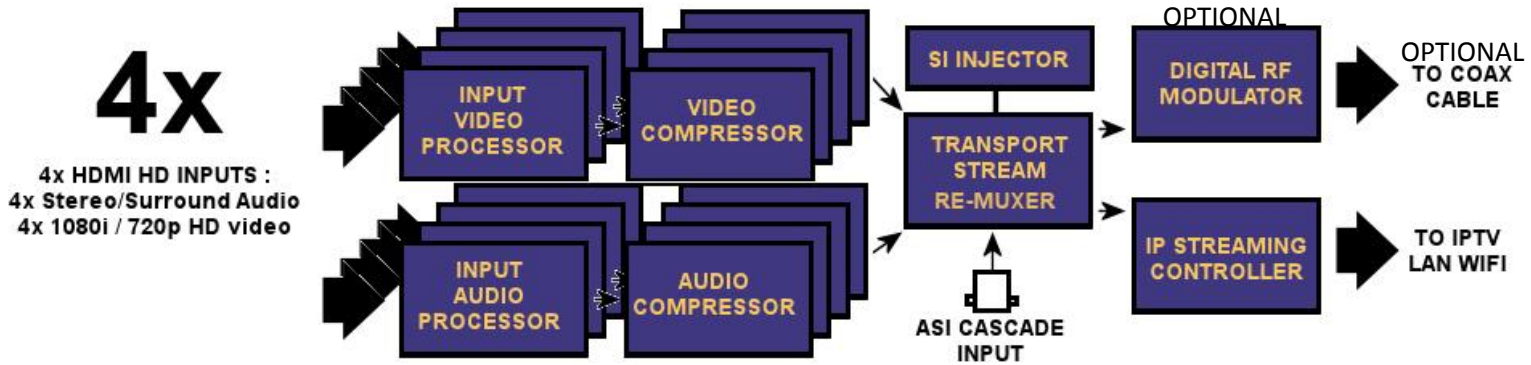
BLOCK DIAGRAM
